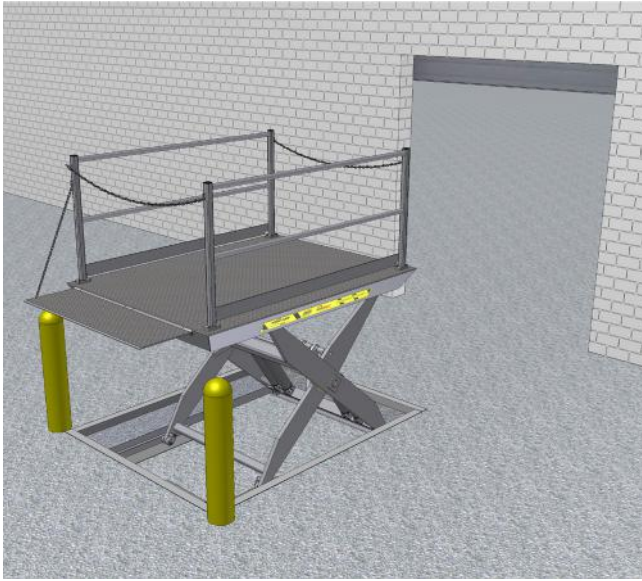
(A) Exterior grade level recessed pit installation
